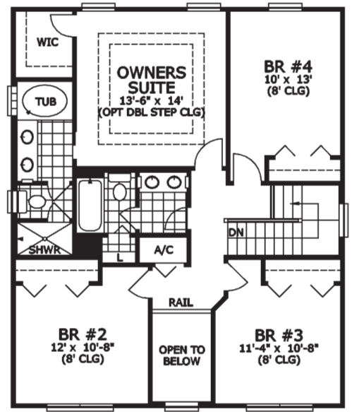
SECOND FLOOR
